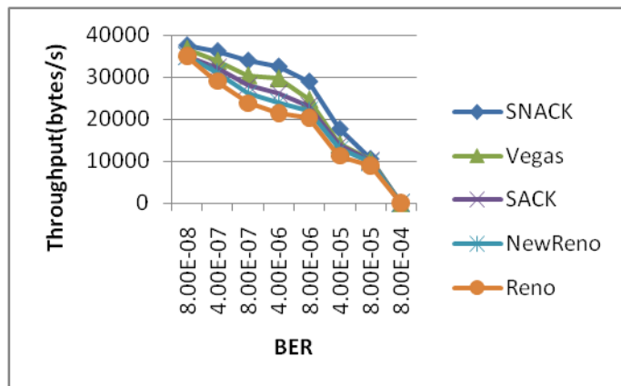
Fig. 3 GEO Satellite Throughput v/s BER
