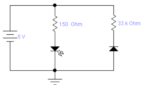
Figure 3. Shows our pulse detection circuit.
