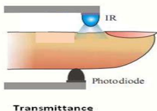
Figure 2. Fingertip sensor
